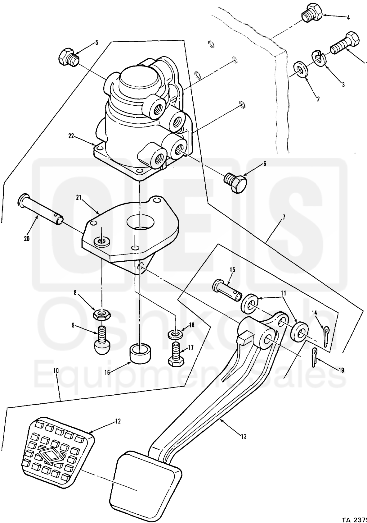
FIGURE 87. BRAKE TREADLE VALVE.
